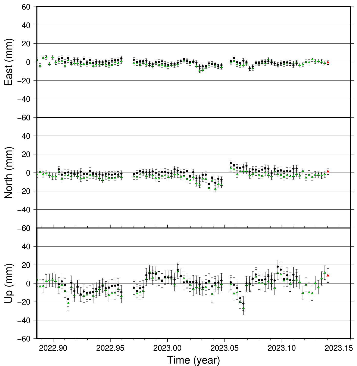
SPBC time series (IGS 2014), last 100 days
