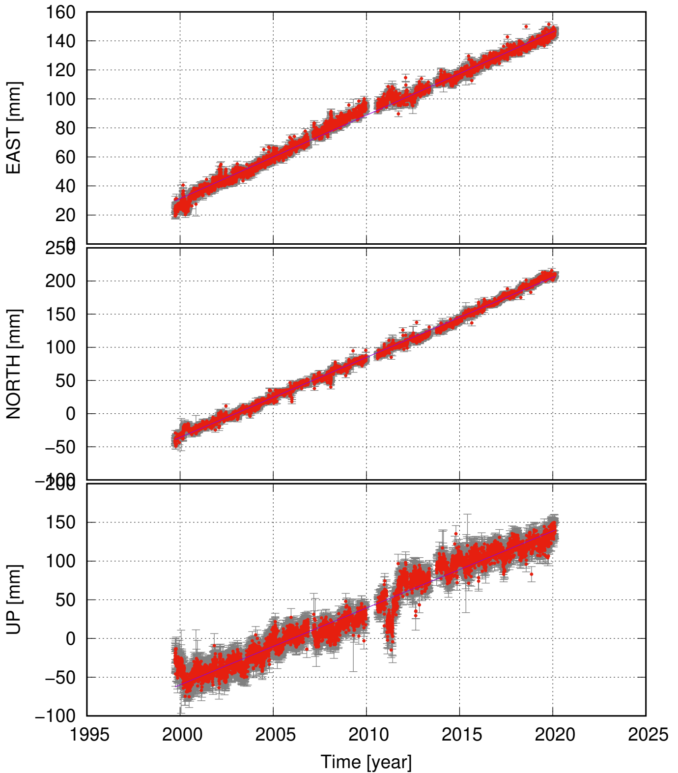
SOHO (63.55, -19.25) time series (ITRF 2014) v_e = 5.75 \pm 0.14 ; v_n = 12.07 \pm 0.19 ; v_u = 9.92 \pm 0.54 mm/yr
