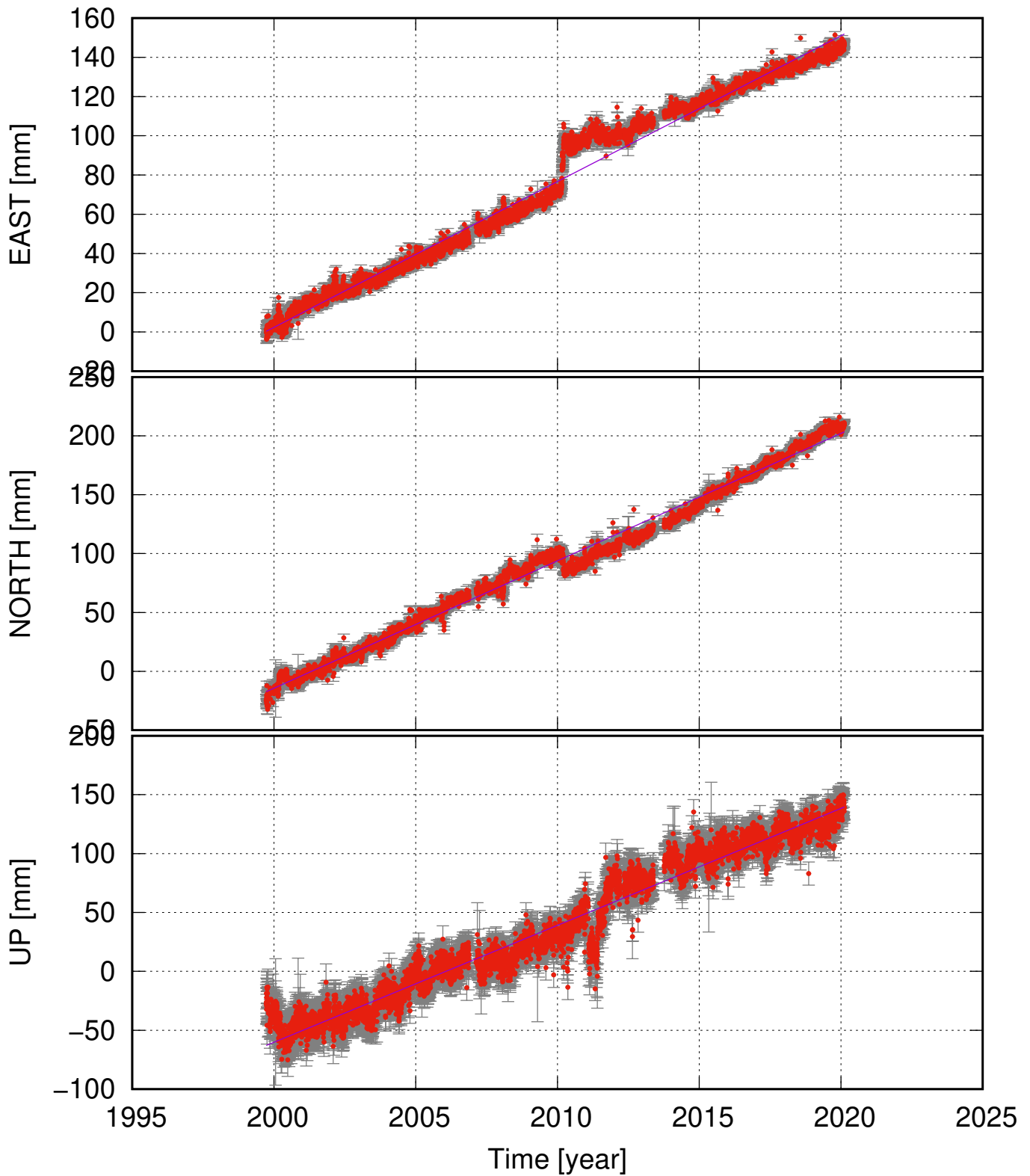
SOHO (63.55, -19.25) time series (ITRF 2014) v_e = 7.43 \pm 0.29 ; v_n = 10.82 \pm 0.30 ; v_u = 9.93 \pm 0.55 mm/yr
