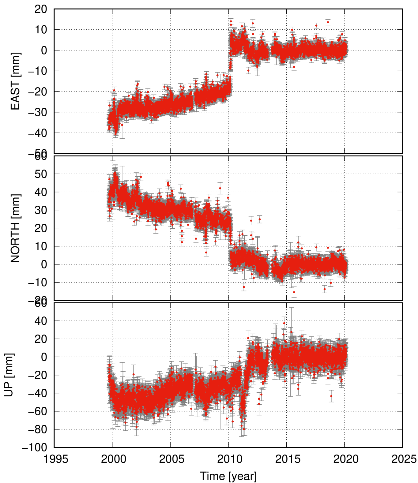
SOHO detrended and seasonal signal removed
