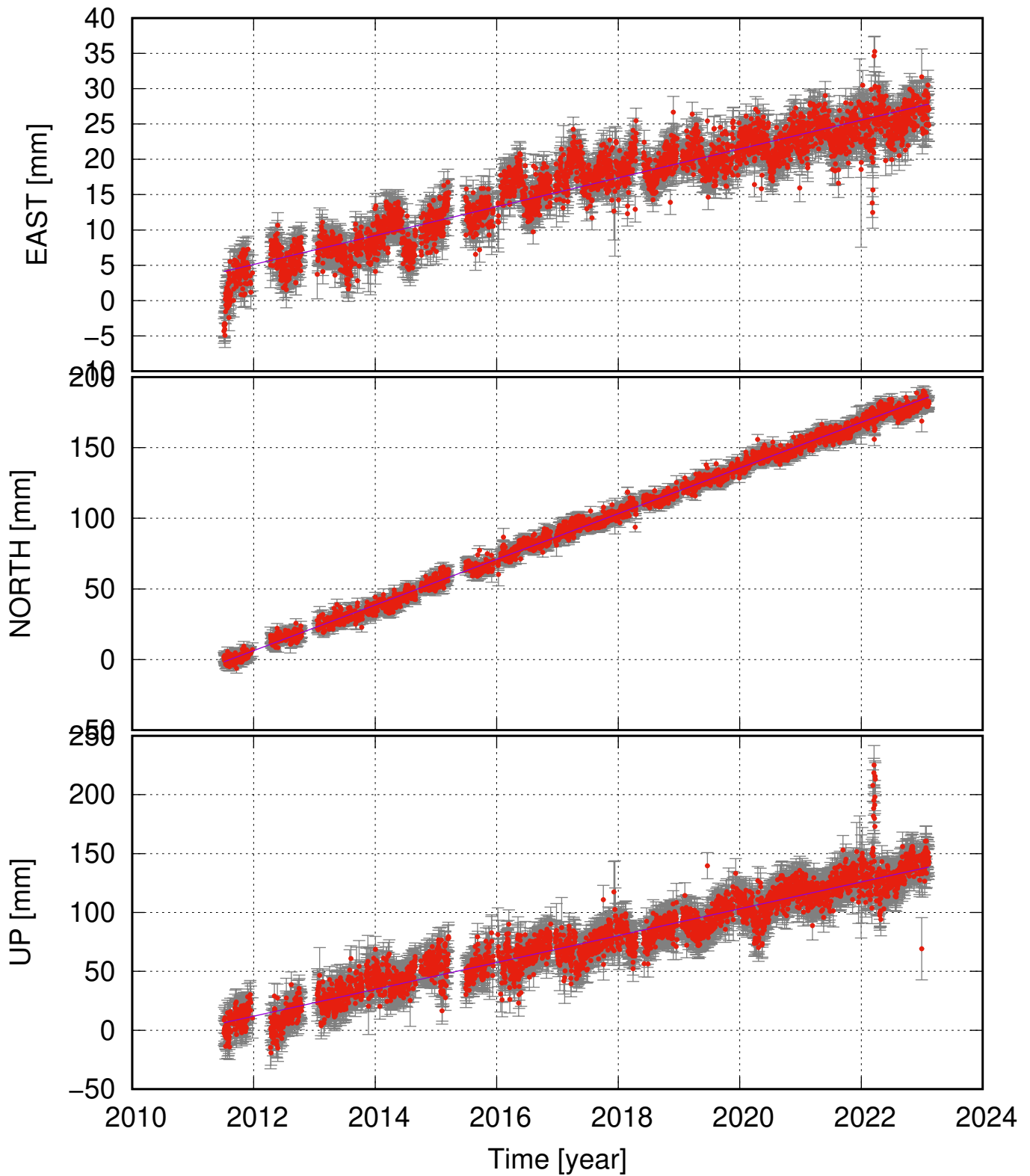
SODU (63.96, -19.59) time series (ITRF 2014) v_e = 2.04 \pm 0.20 ; v_n = 16.16 \pm 0.28 ; v_u = 11.39 \pm 0.94 mm/yr
