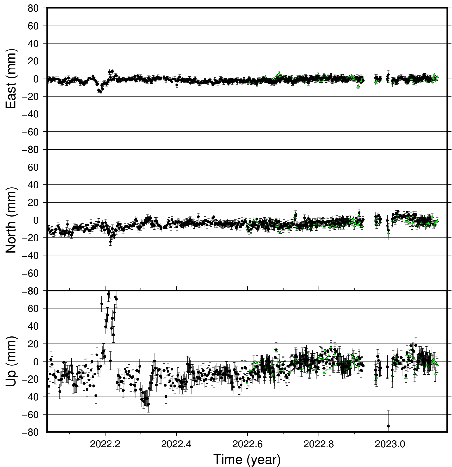
SODU time series (IGS 2014), last 400 days
