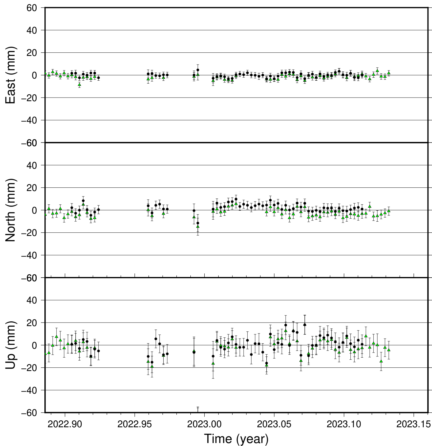
SODU time series (IGS 2014), last 100 days
