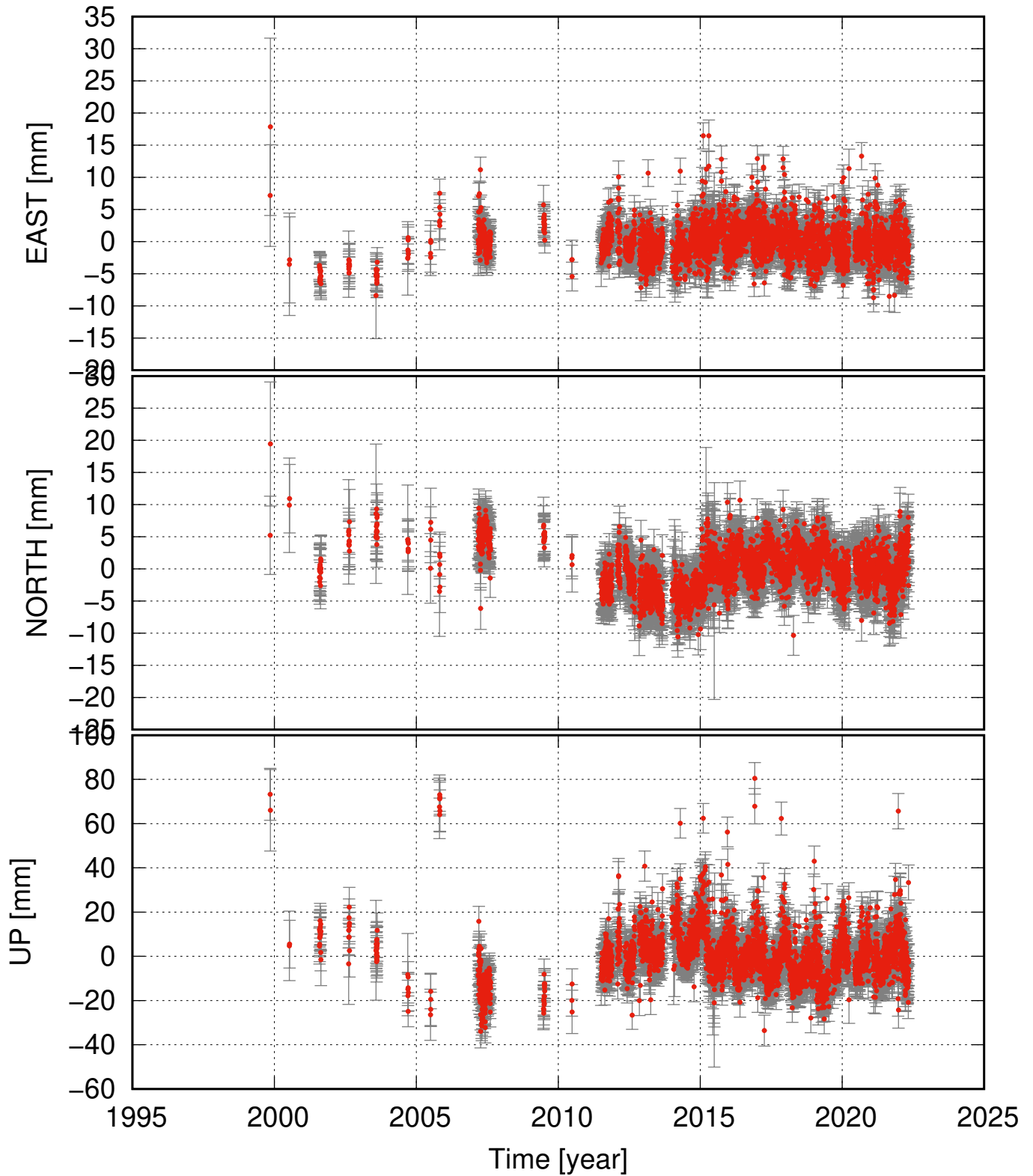
SNAE residual time series (some major events removed as well)
