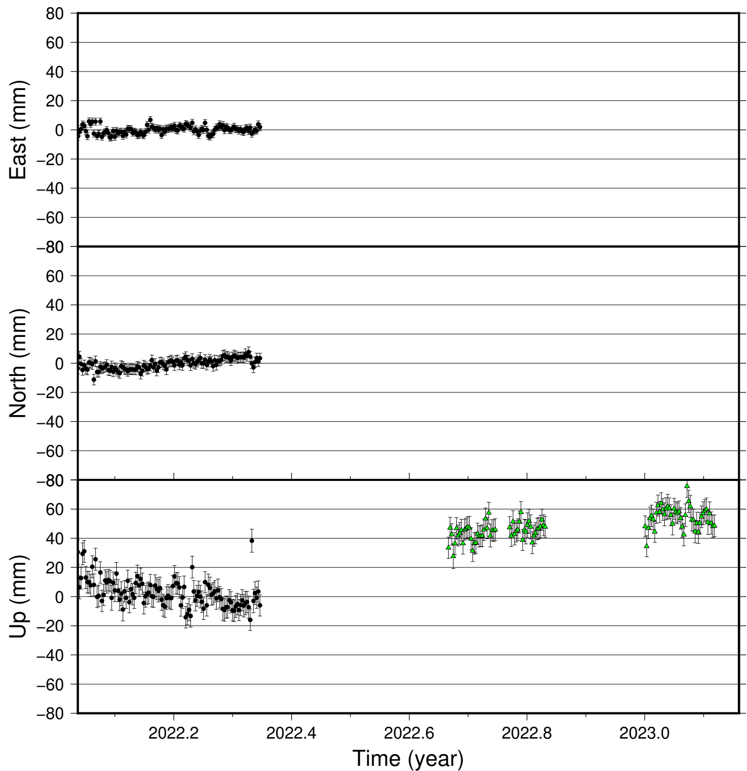
SNAE time series (IGS 2014), last 400 days
