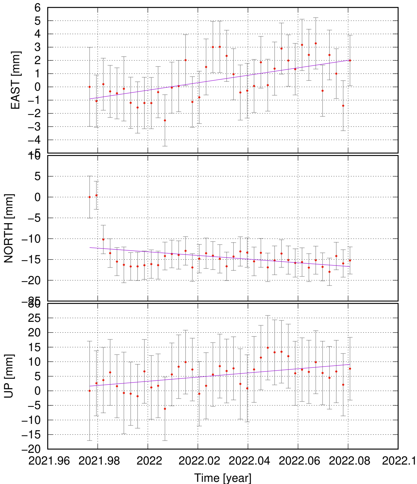
SLEI (63.88, -22.23) time series (ITRF 2014) v_e = 28.14 \pm 12.89 ; v_n = -43.77 \pm 32.95 ; v_u = 71.53 \pm 39.33 mm/yr
