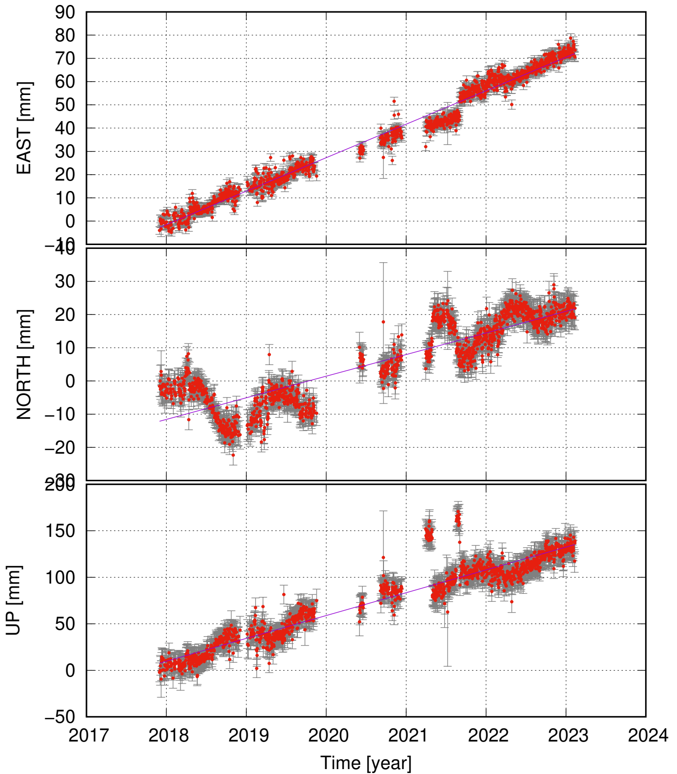
SLEC (63.94, -16.63) time series (ITRF 2014) v_e = 14.40 \pm 0.62 ; v_n = 6.51 \pm 1.11 ; v_u = 24.54 \pm 2.75 mm/yr
