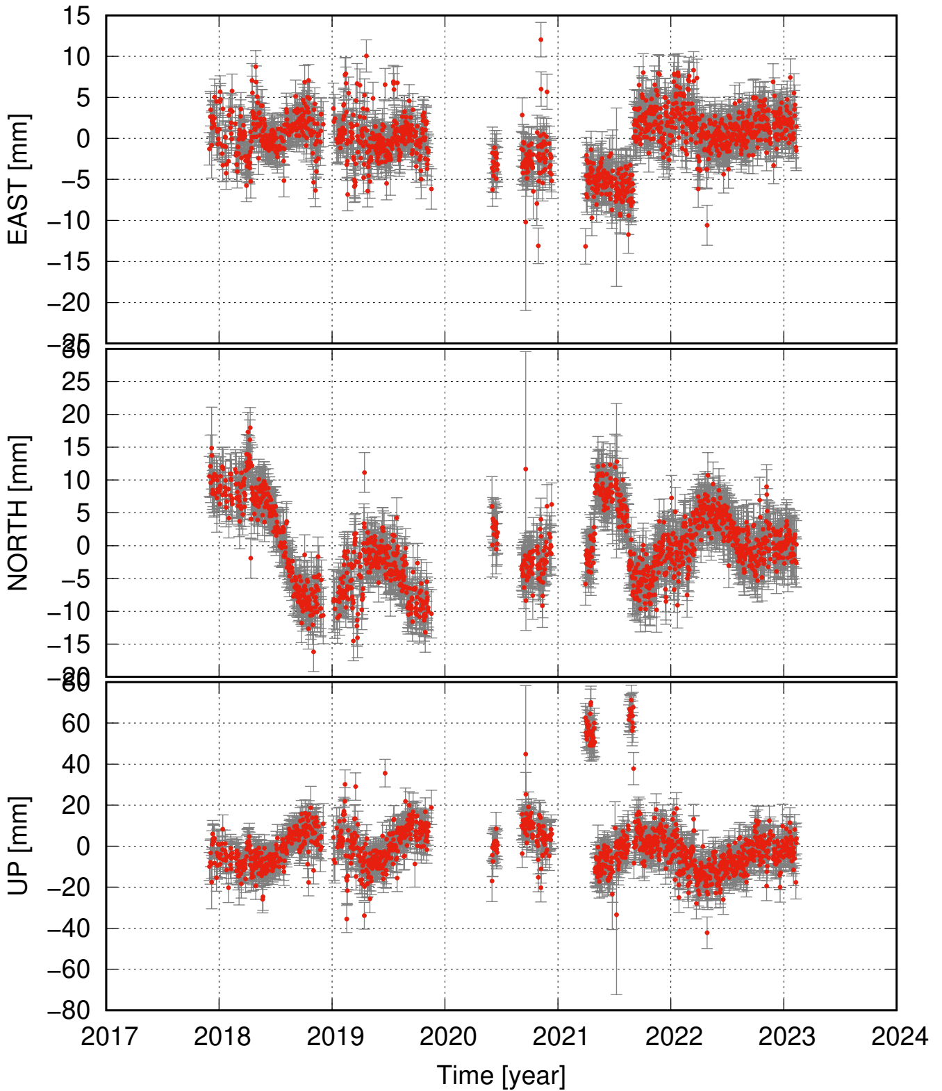
SLEC residual time series (some major events removed as well)
