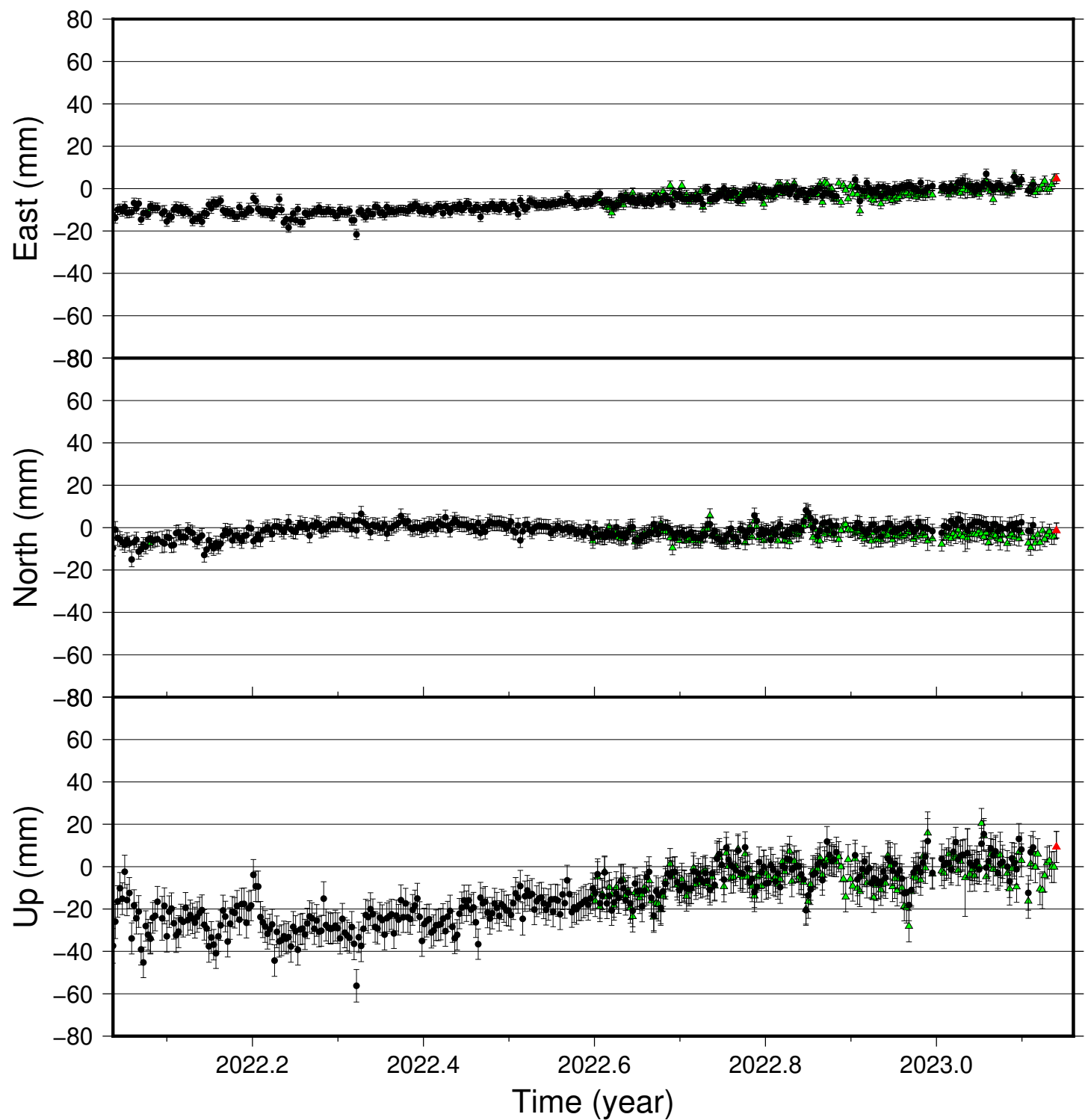
SLEC time series (IGS 2014), last 400 days
