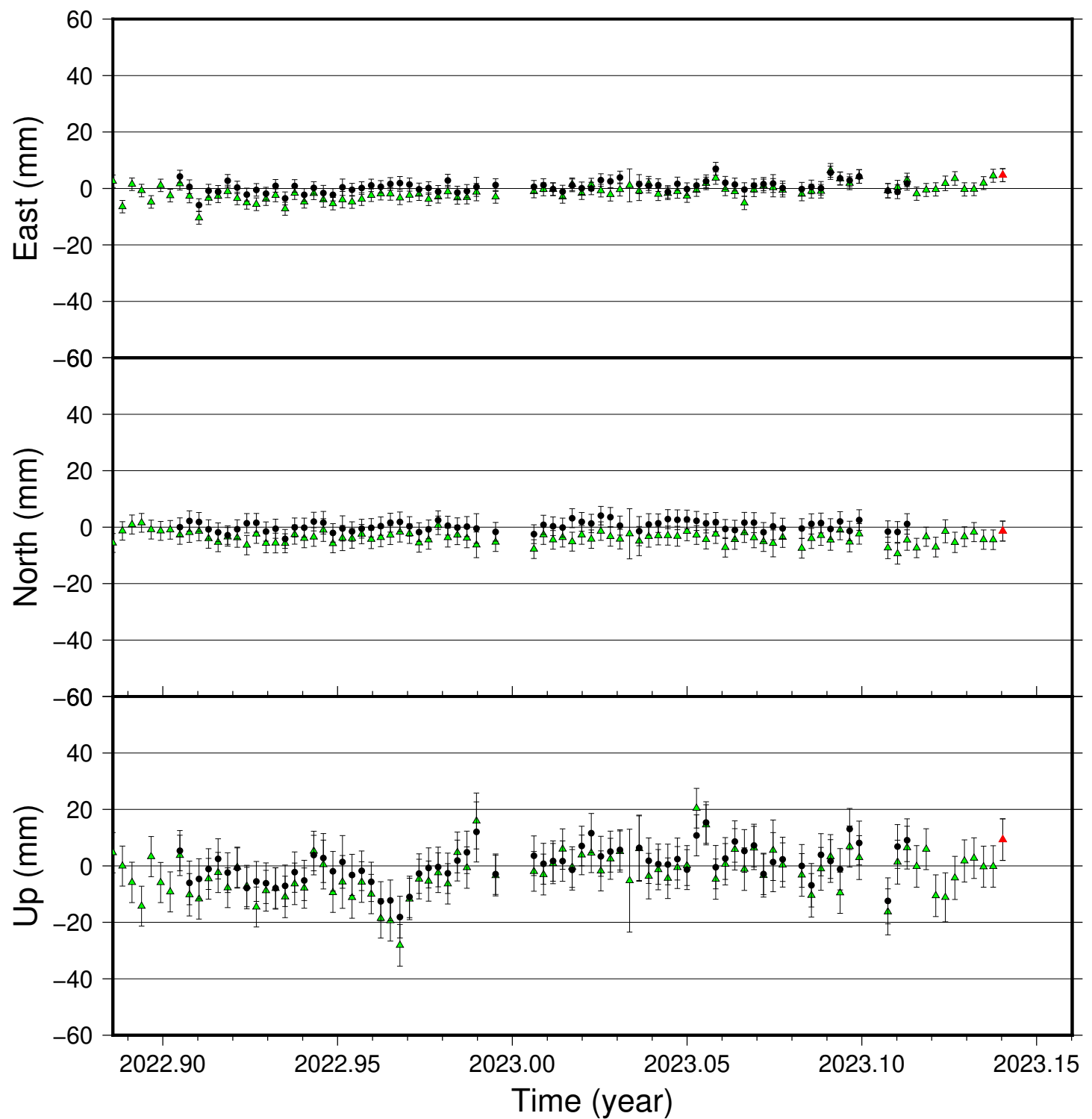
SLEC time series (IGS 2014), last 100 days
