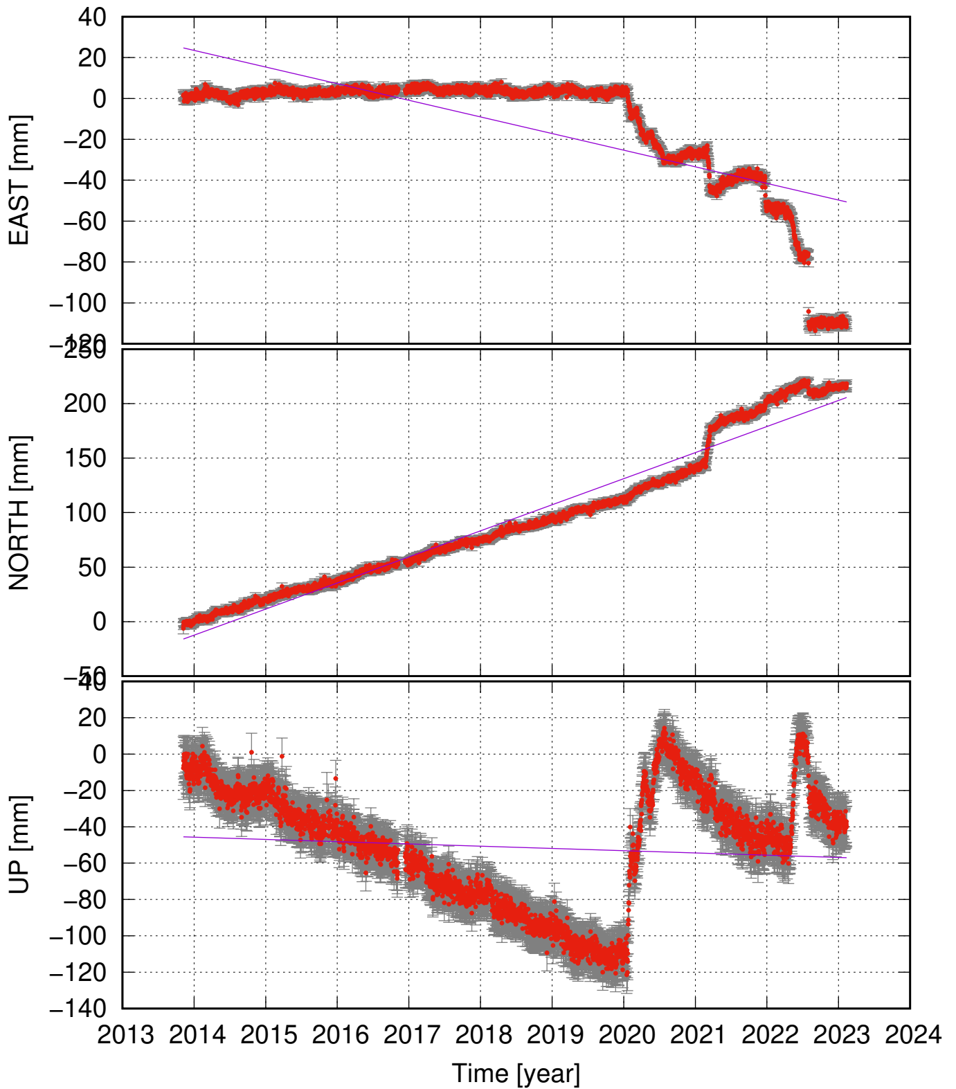
SKSH (63.87, -22.48) time series (ITRF 2014) v_e = -8.14 \pm 2.21 ; v_n = 23.93 \pm 1.42 ; v_u = -1.25 \pm 3.50 mm/yr
