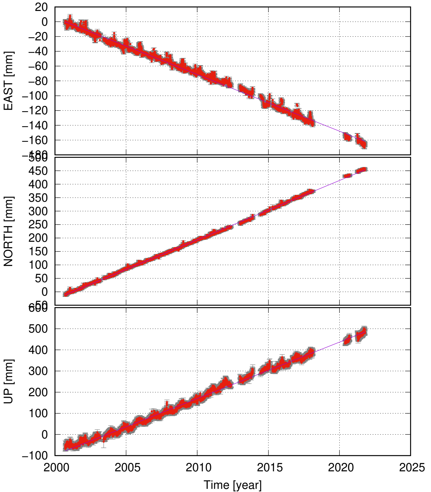
SKRO (64.56, -18.38) time series (ITRF 2014) v_e = -7.67 \pm 0.16 ; v_n = 22.04 \pm 0.15 ; v_u = 26.69 \pm 0.54 mm/yr
