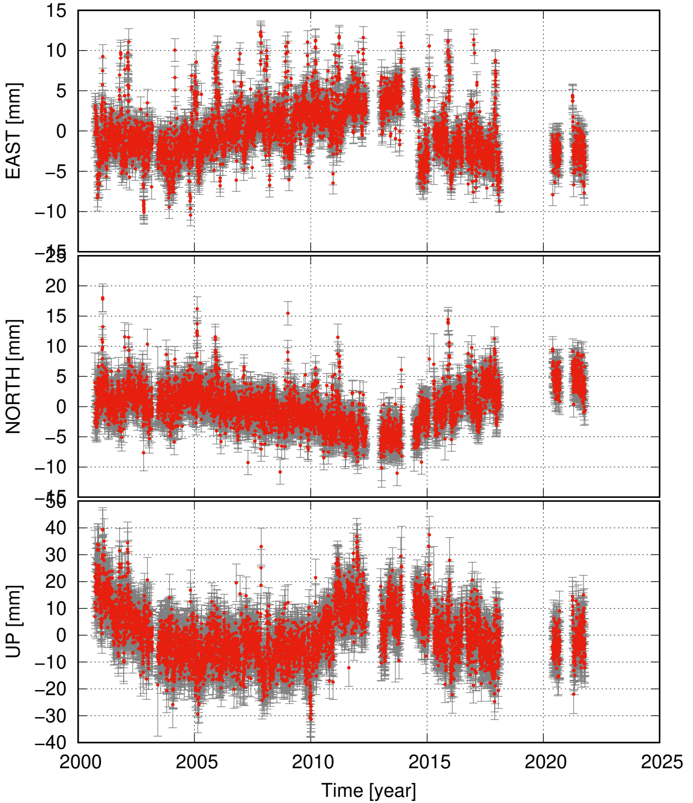
SKRO detrended and seasonal signal removed
