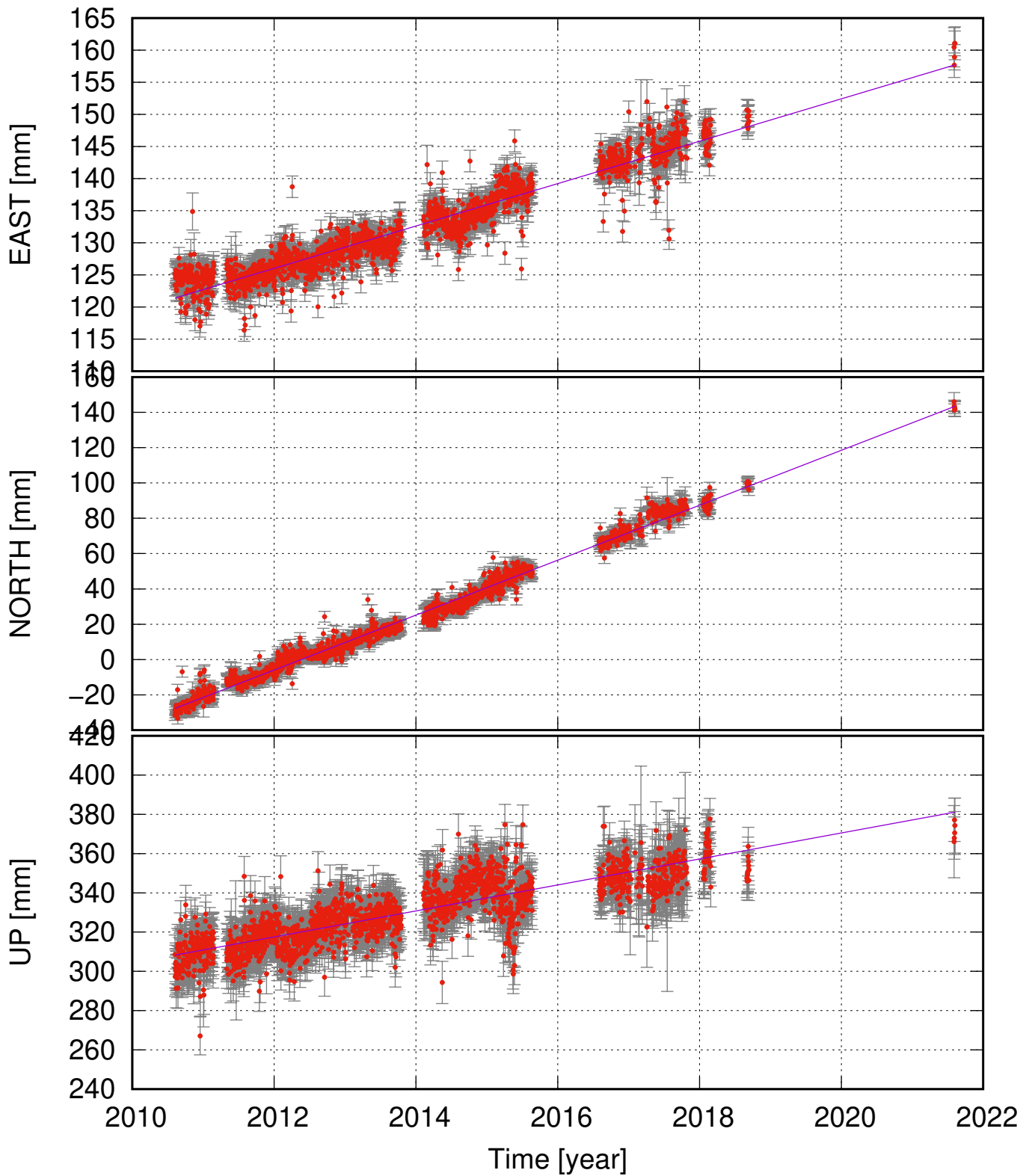
SKOG (63.58, -19.45) time series (ITRF 2014) v_e = 3.30 \pm 0.20 ; v_n = 15.55 \pm 0.33 ; v_u = 6.62 \pm 0.81 mm/yr
