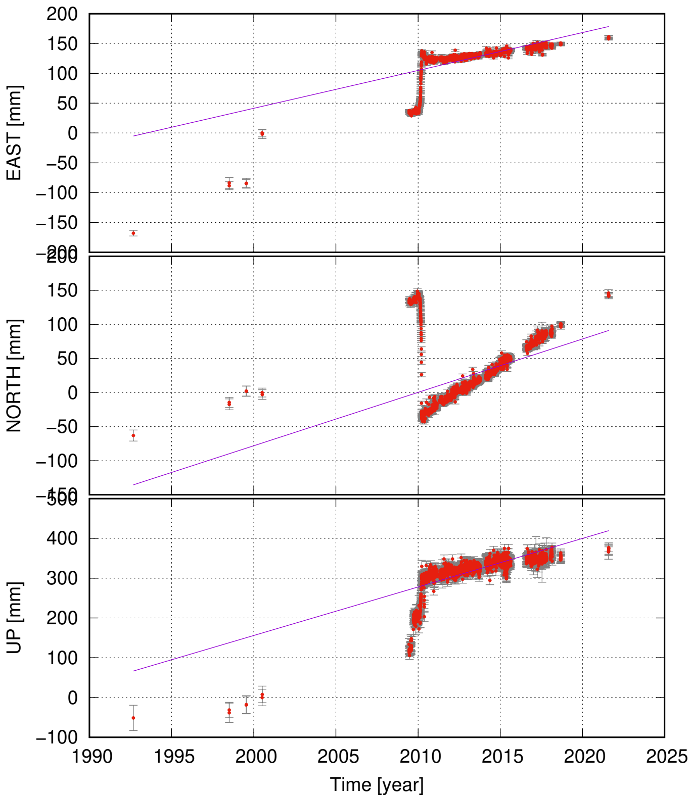
SKOG (63.58, -19.45) time series (ITRF 2014) v_e = 6.34 \pm 0.68 ; v_n = 7.83 \pm 1.41 ; v_u = 12.19 \pm 1.06 mm/yr
