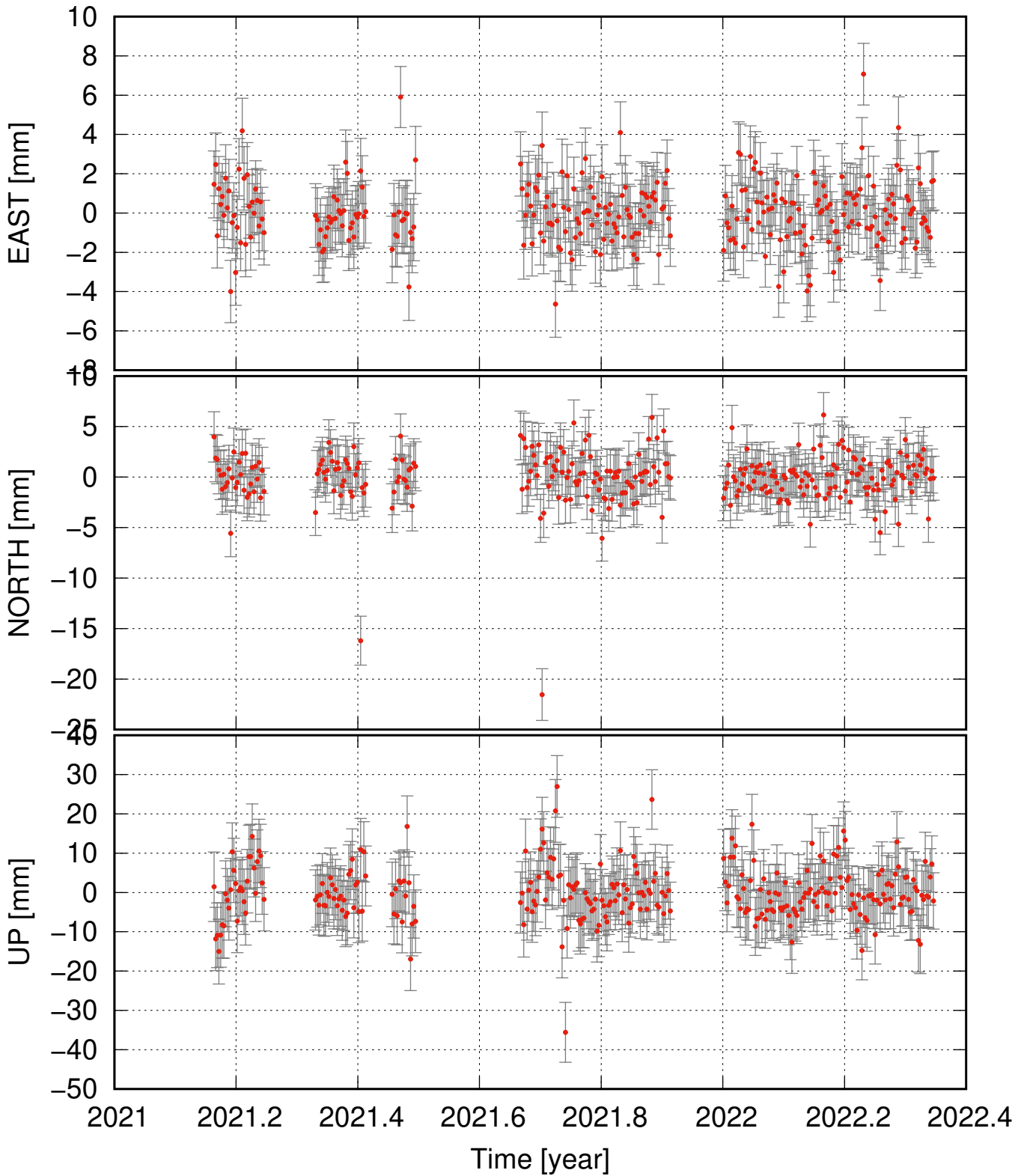
SKHA detrended and seasonal signal removed
