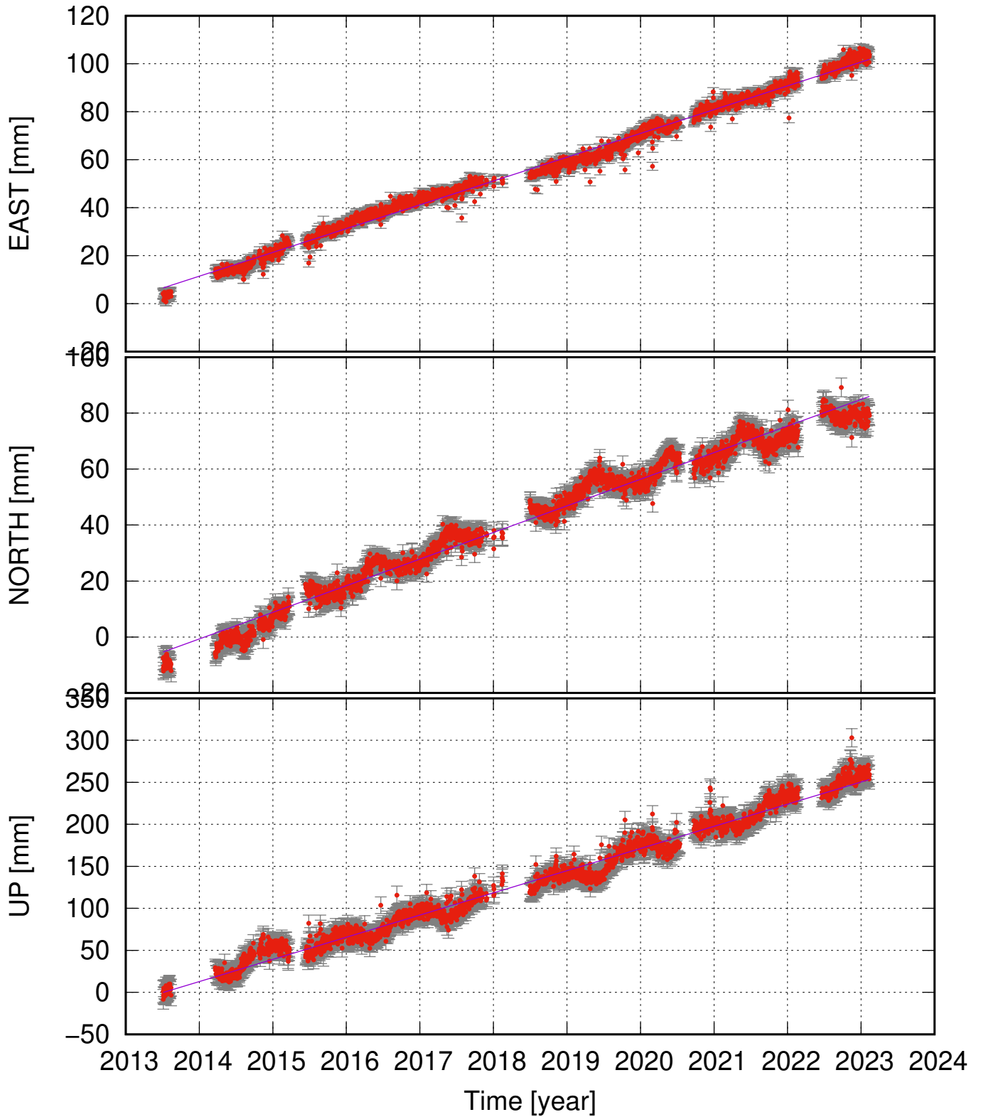
SKFC (64.03, -16.99) time series (ITRF 2014) v_e = 9.91 \pm 0.25 ; v_n = 9.51 \pm 0.38 ; v_u = 26.40 \pm 0.98 mm/yr
