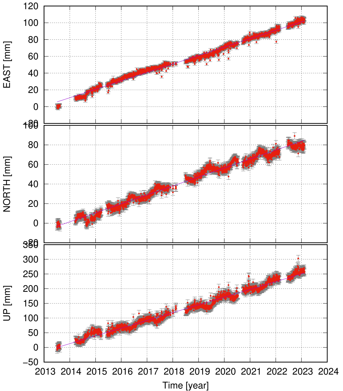
SKFC (64.03, -16.99) time series (ITRF 2014) v_e = 10.05 \pm 0.28 ; v_n = 9.16 \pm 0.35 ; v_u = 26.40 \pm 0.98 mm/yr
