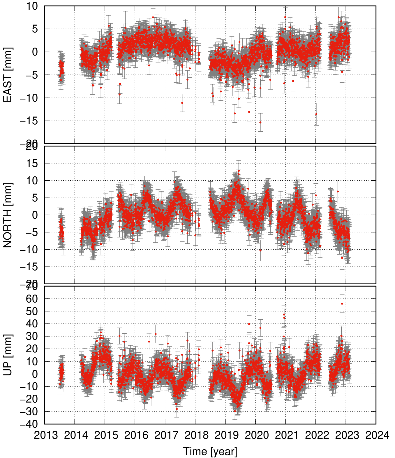
SKFC residual time series (some major events removed as well)
