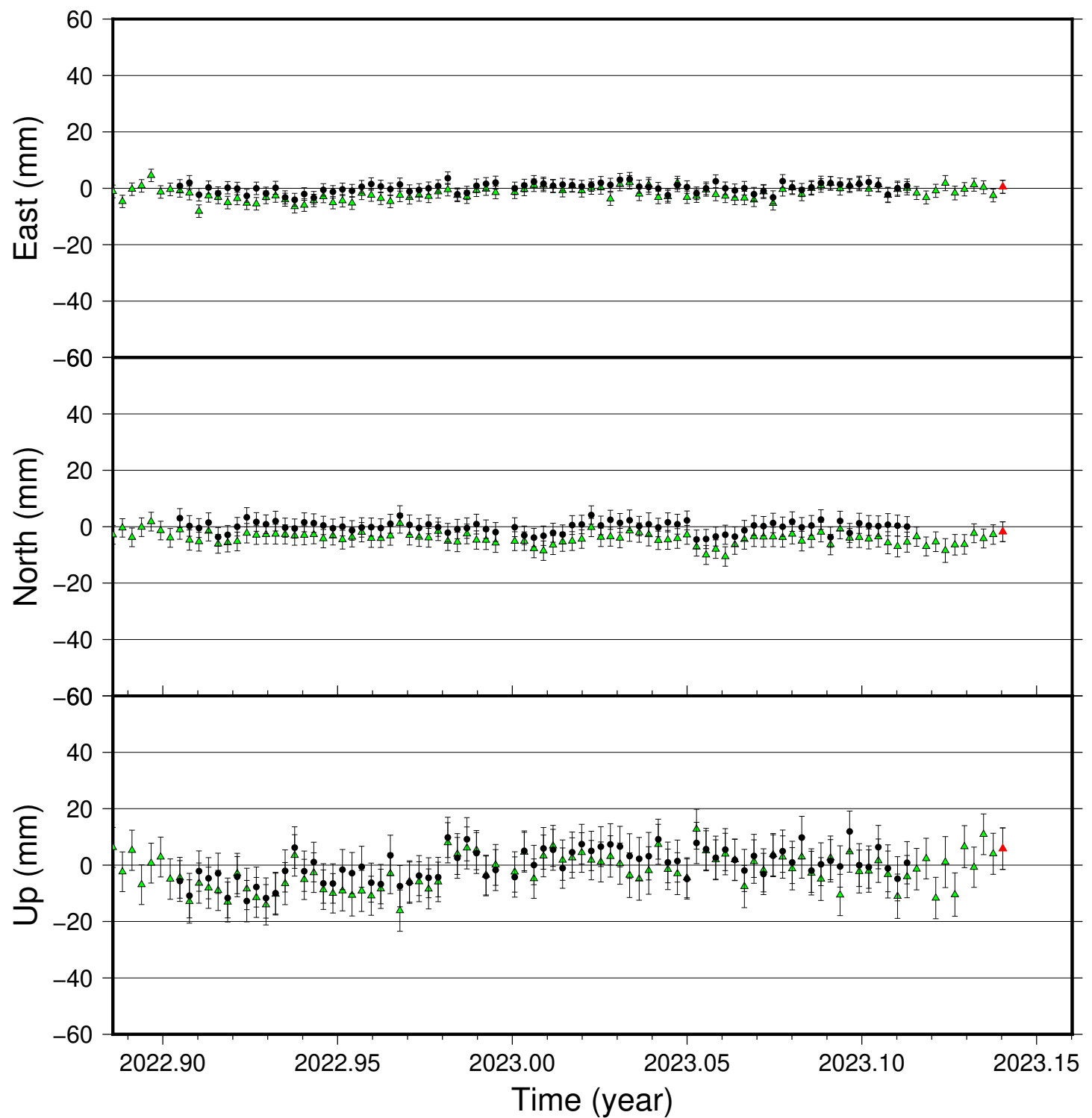
SKFC time series (IGS 2014), last 100 days
