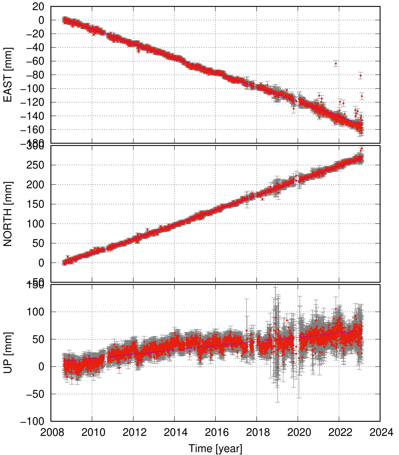
SKDA (64.38, -20.67) time series (ITRF 2014) v_e = -10.64 \pm 0.21 ; v_n = 18.65 \pm 0.20 ; v_u = 3.86 \pm 0.70 mm/yr
