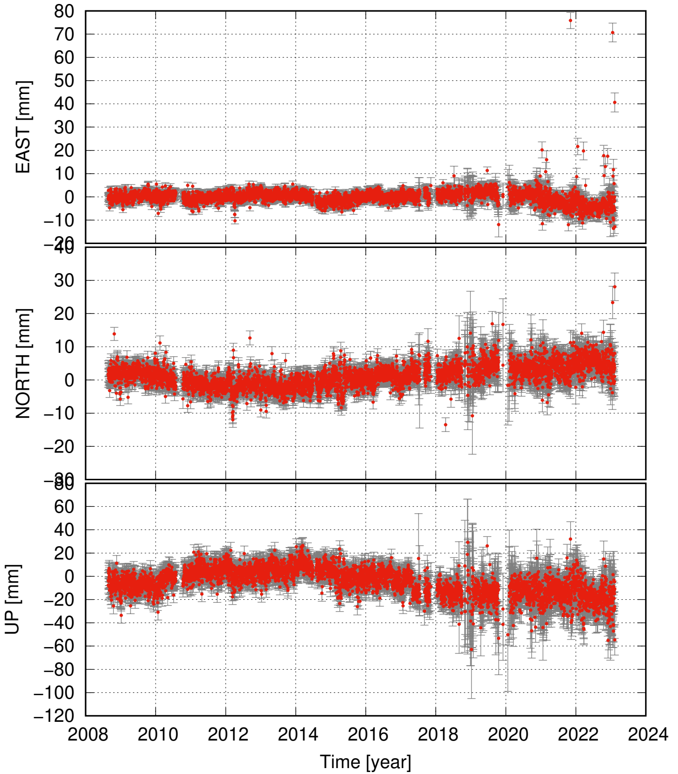
SKDA detrended and seasonal signal removed
