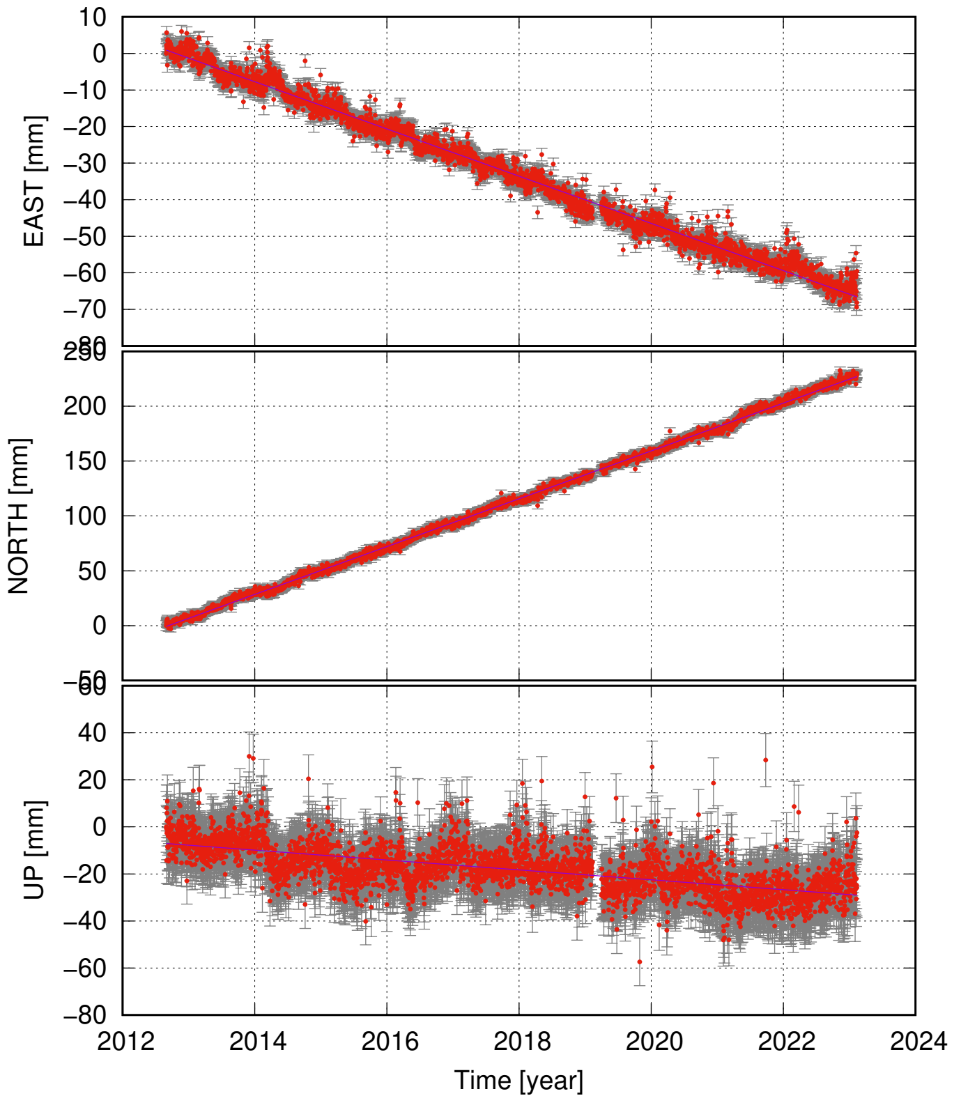
SJUK (66.05, -17.34) time series (ITRF 2014) v_e = -6.46 \pm 0.21 ; v_n = 21.80 \pm 0.22 ; v_u = -2.09 \pm 0.72 mm/yr
