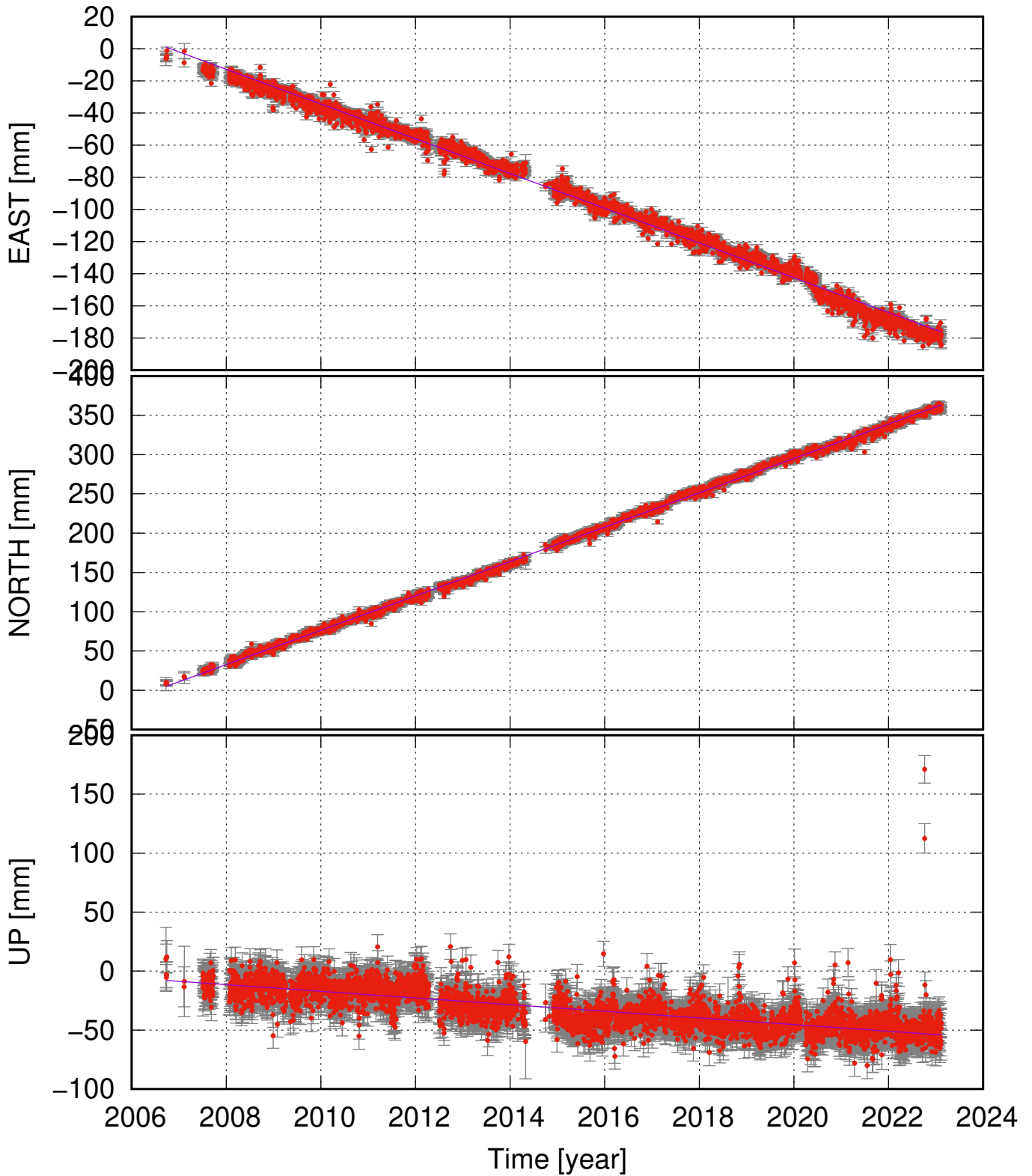
SIFJ (66.14, -18.90) time series (ITRF 2014) v_e = -10.81 \pm 0.23 ; v_n = 21.87 \pm 0.20 ; v_u = -2.81 \pm 0.63 mm/yr
