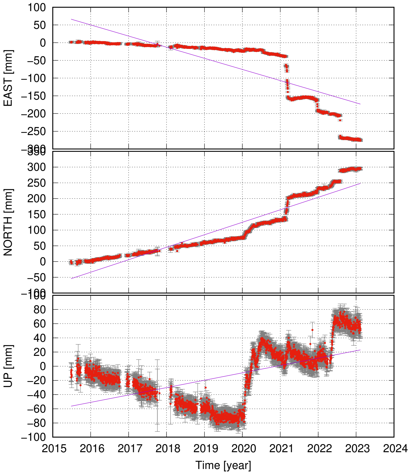
SENG (63.88, -22.43) time series (ITRF 2014) ve = -31.40 ± 6.77; vn = 39.62 ± 4.08; vu = 10.40 ± 4.47 mm/yr
