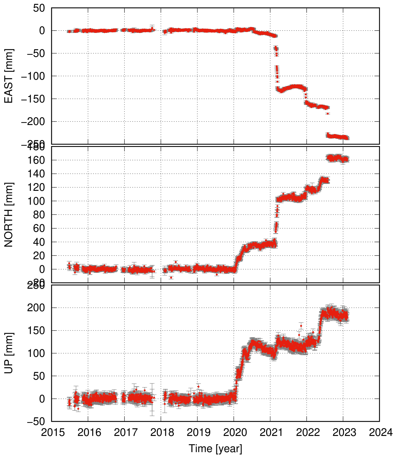
SENG detrended and seasonal signal removed
