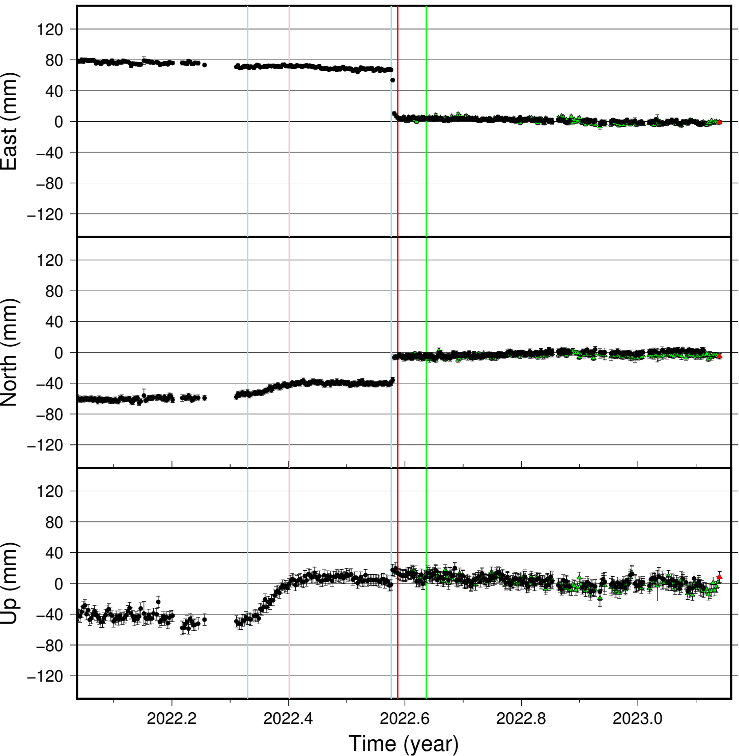
SENG time series (IGS 2014), last 400 days
