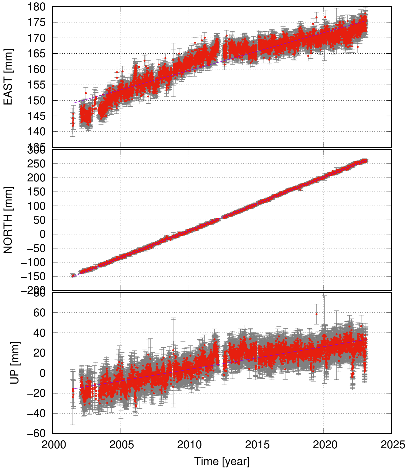
SELF (63.93, -21.03) time series (ITRF 2014) v_e = 1.22 \pm 0.12 ; v_n = 19.13 \pm 0.10 ; v_u = 2.27 \pm 0.32 mm/yr
