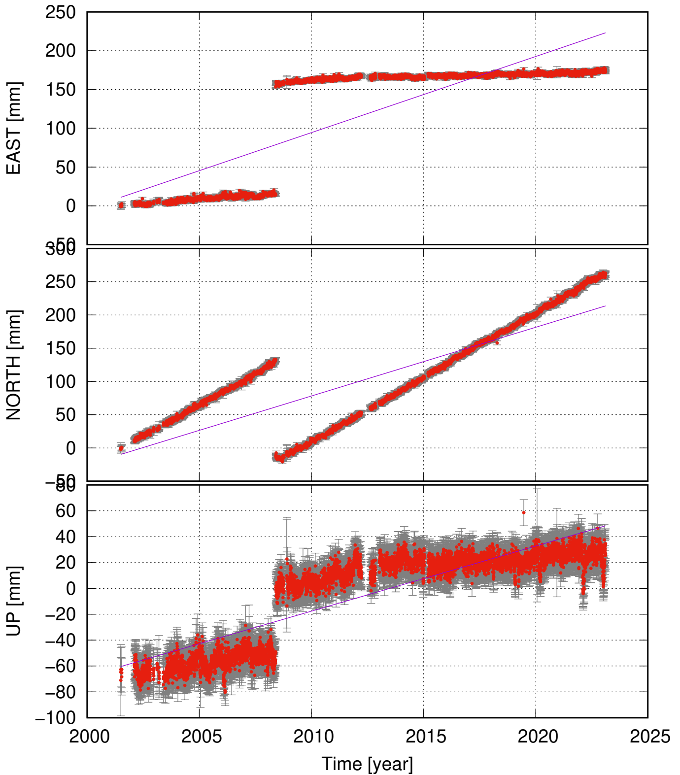
SELF (63.93, -21.03) time series (ITRF 2014) v_e = 9.81 \pm 1.91 ; v_n = 10.33 \pm 1.95 ; v_u = 5.03 \pm 0.79 mm/yr
