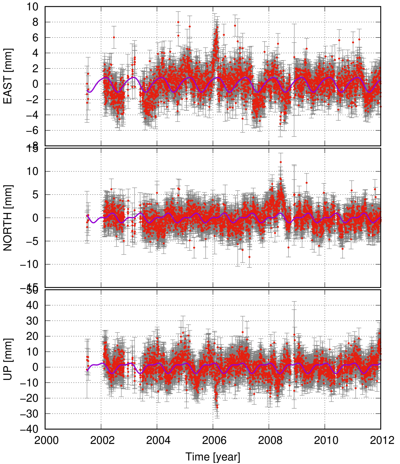
SELF seasonal fit
