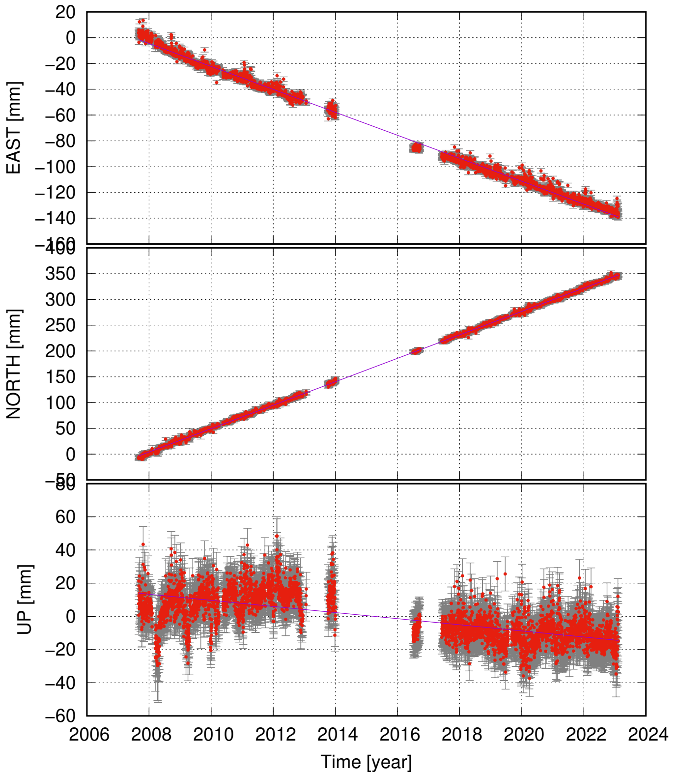
SAVI (65.99, -17.38) time series (ITRF 2014) v_e = -8.90 \pm 0.17 ; v_n = 22.72 \pm 0.14 ; v_u = -1.84 \pm 0.62 mm/yr
