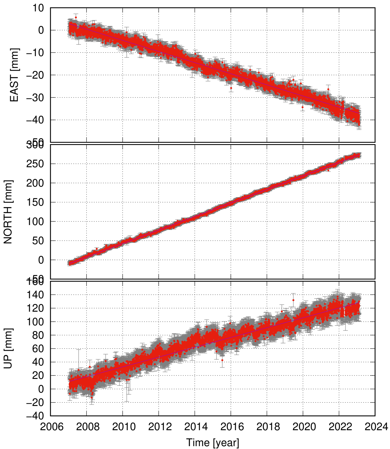
SAUR (63.98, -20.43) time series (ITRF 2014) v_e = -2.48 \pm 0.09 ; v_n = 17.58 \pm 0.14 ; v_u = 7.29 \pm 0.41 mm/yr
