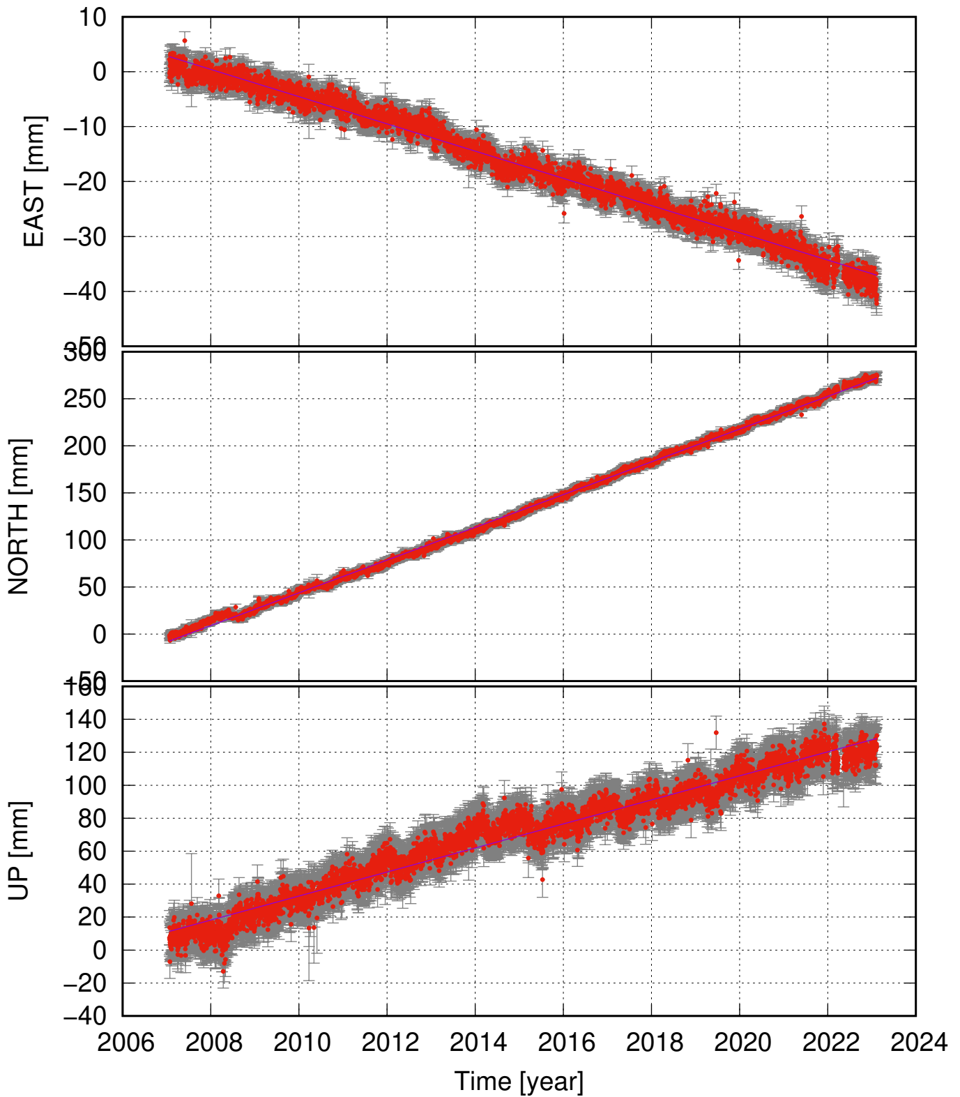
SAUR (63.98, -20.43) time series (ITRF 2014) v_e = -2.48 \pm 0.09 ; v_n = 17.39 \pm 0.18 ; v_u = 7.29 \pm 0.41 mm/yr
