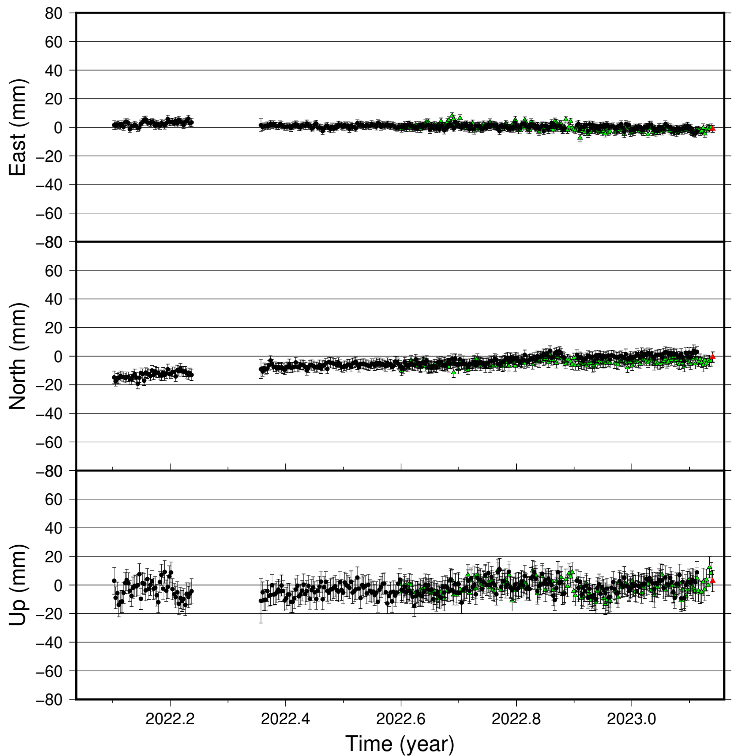
SAUR time series (IGS 2014), last 400 days
