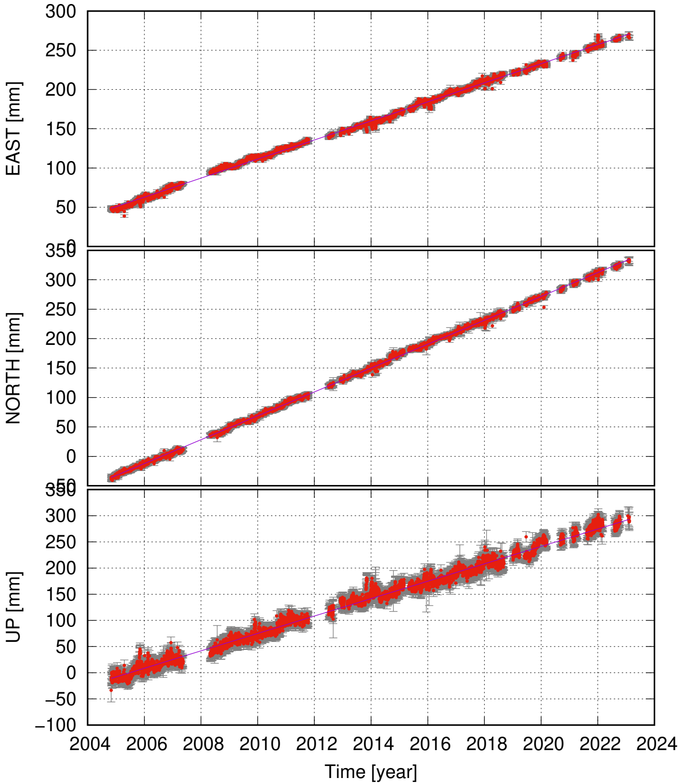
SAUD (64.90, -15.88) time series (ITRF 2014) ve = 12.15 ± 0.15; vn = 20.29 ± 0.13; vu = 16.63 ± 0.44 mm/yr
