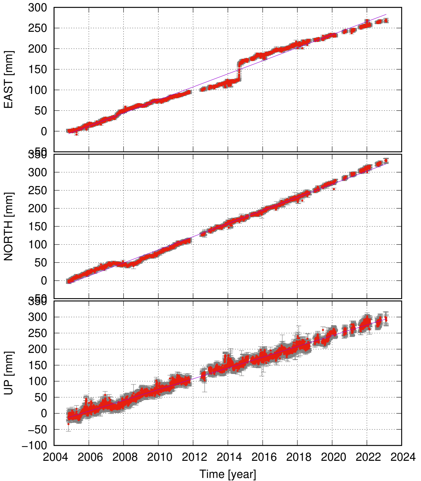
SAUD (64.90, -15.88) time series (ITRF 2014) ve = 15.83 ± 0.56; vn = 18.14 ± 0.37; vu = 16.78 ± 0.46 mm/yr
