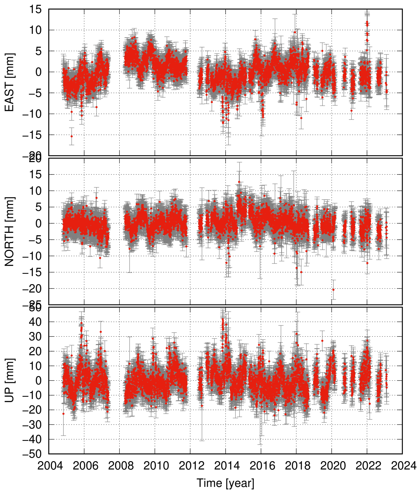
SAUD residual time series (some major events removed as well)
