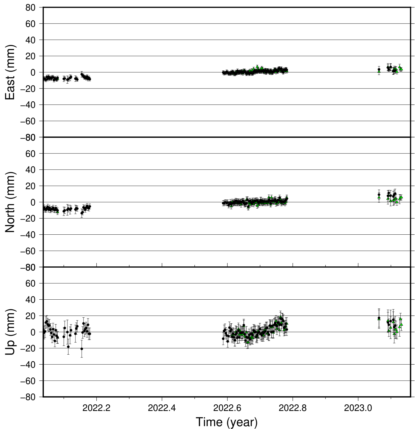
SAUD time series (IGS 2014), last 400 days
