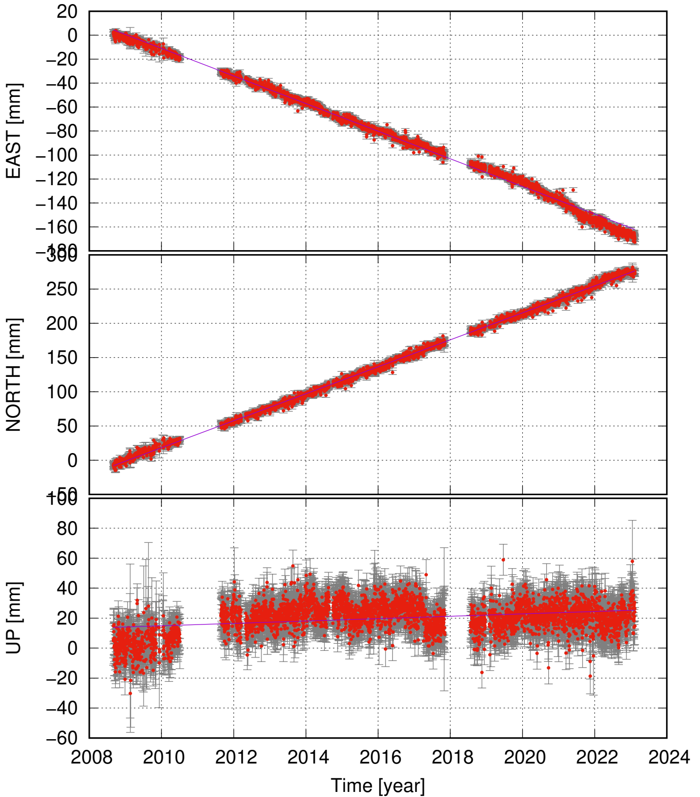
SARP (64.47, -21.27) time series (ITRF 2014) v_e = -11.52 \pm 0.22 ; v_n = 19.69 \pm 0.22 ; v_u = 0.79 \pm 0.64 mm/yr
