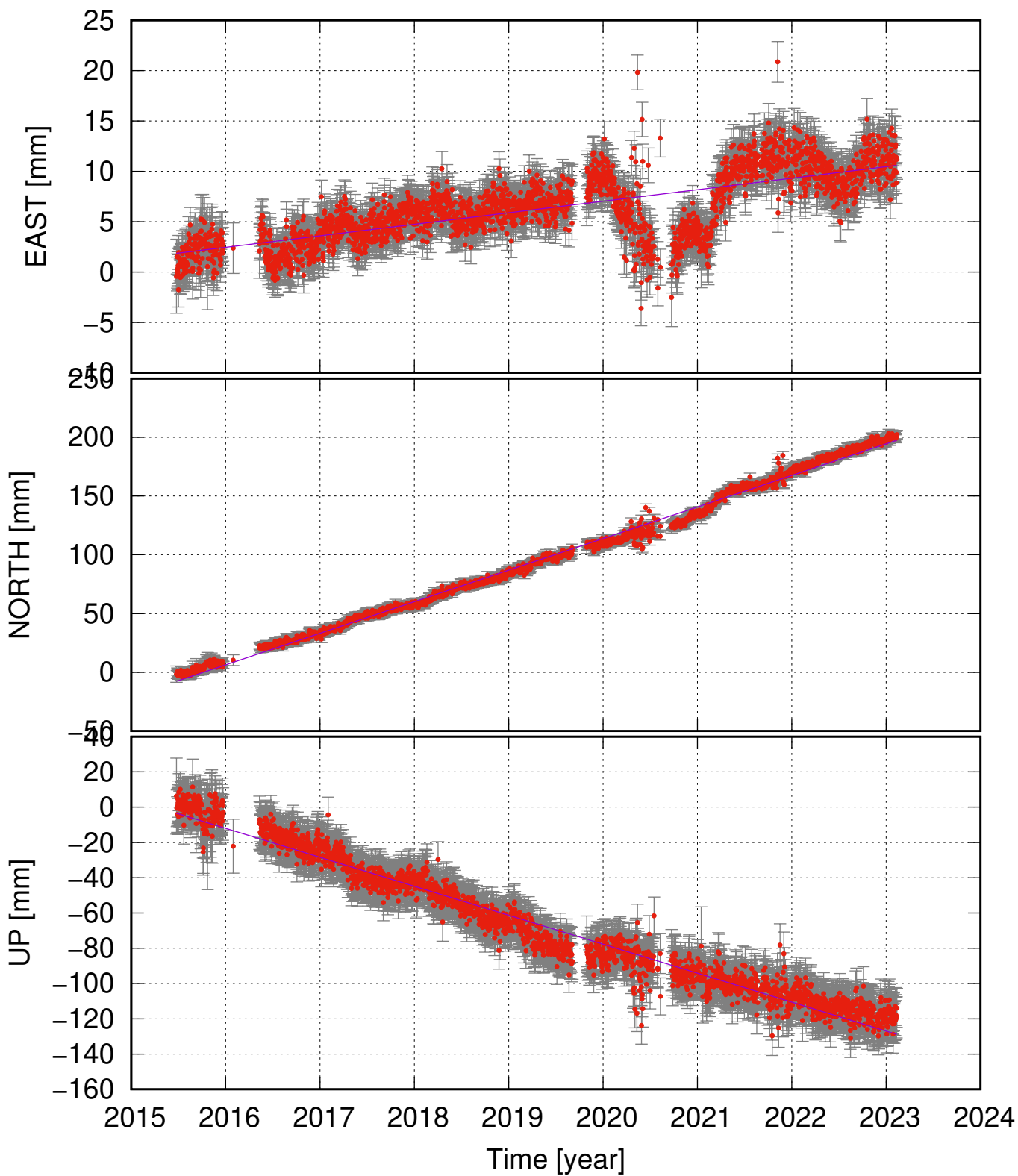
RVIT (63.82, -22.70) time series (ITRF 2014) v_e = 1.14 \pm 0.30 ; v_n = 26.88 \pm 0.54 ; v_u = -16.42 \pm 0.90 mm/yr
