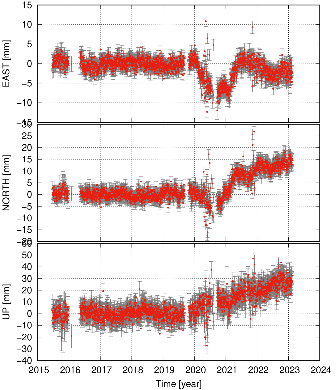
RVIT detrended and seasonal signal removed
