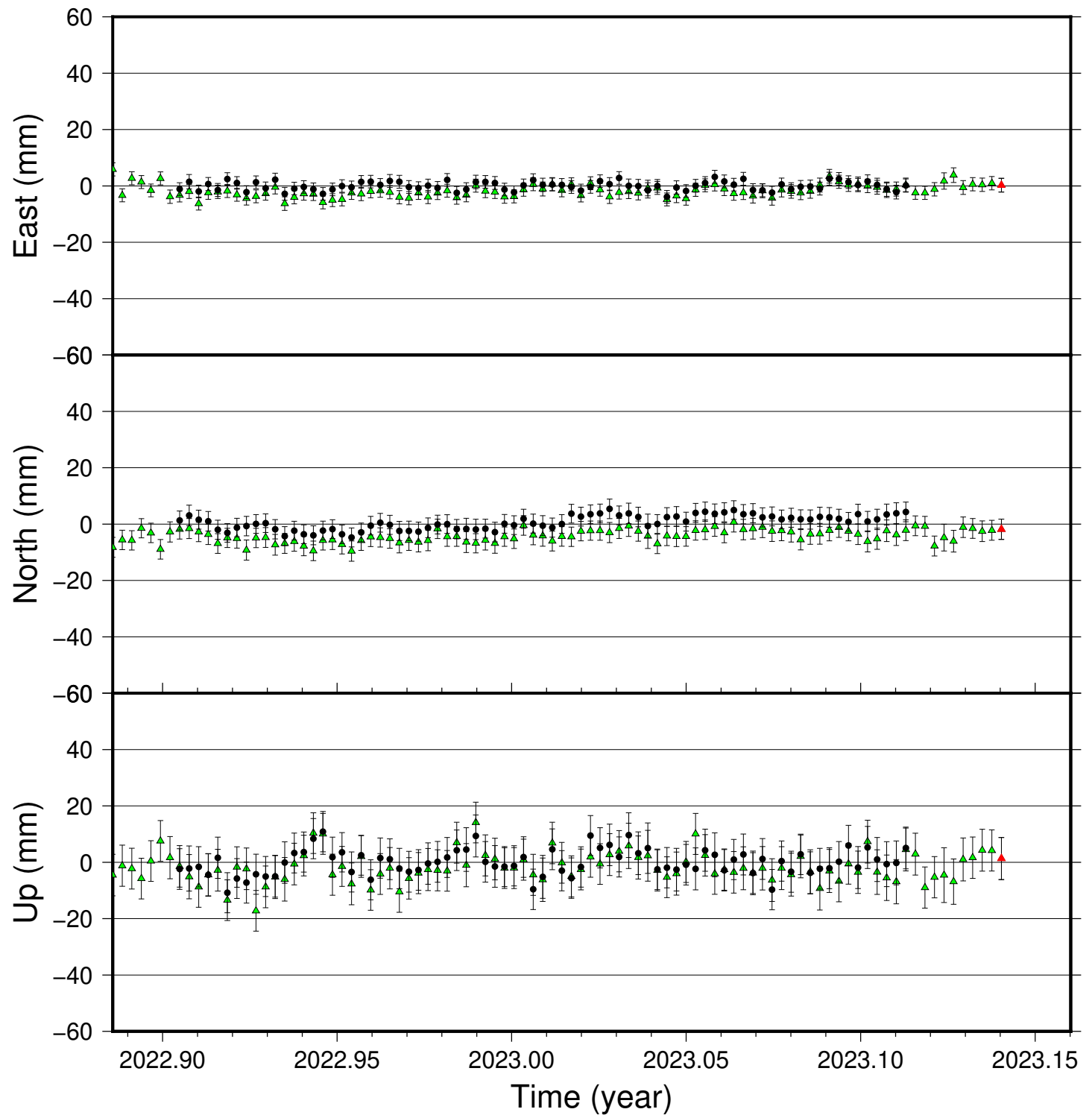
RVIT time series (IGS 2014), last 100 days
