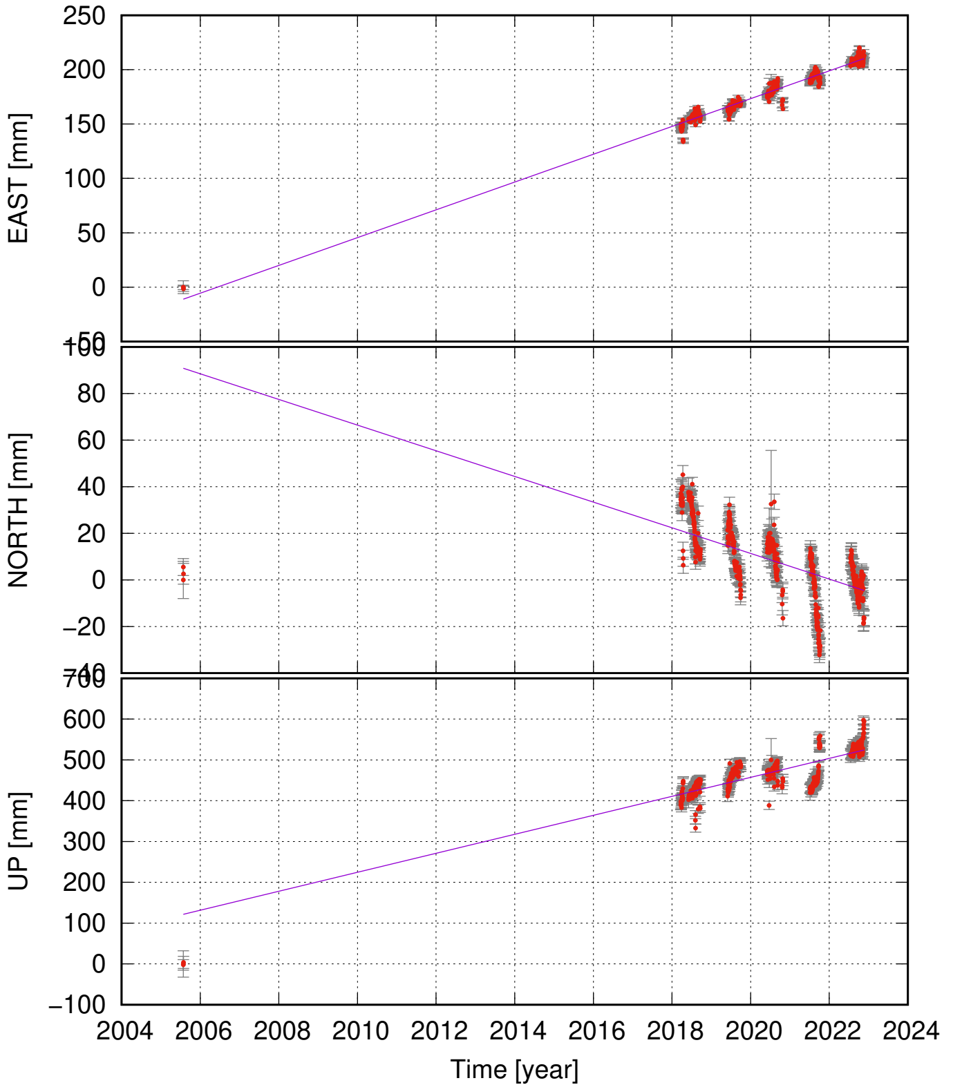
ROTH (63.98, -16.66) time series (ITRF 2014) v_e = 12.78 \pm 0.23 ; v_n = -5.51 \pm 0.71 ; v_u = 23.24 \pm 1.71 mm/yr
