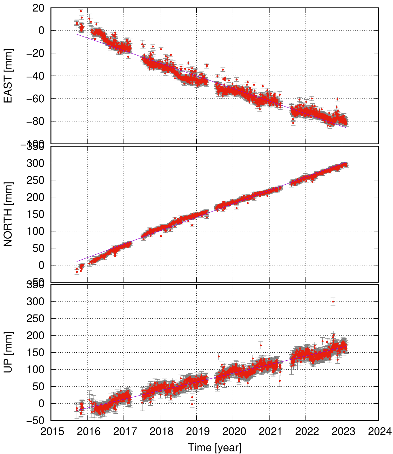
RJUC (64.74, -17.53) time series (ITRF 2014) v_e = -11.13 \pm 0.58 ; v_n = 39.52 \pm 0.99 ; v_u = 25.44 \pm 1.44 mm/yr
