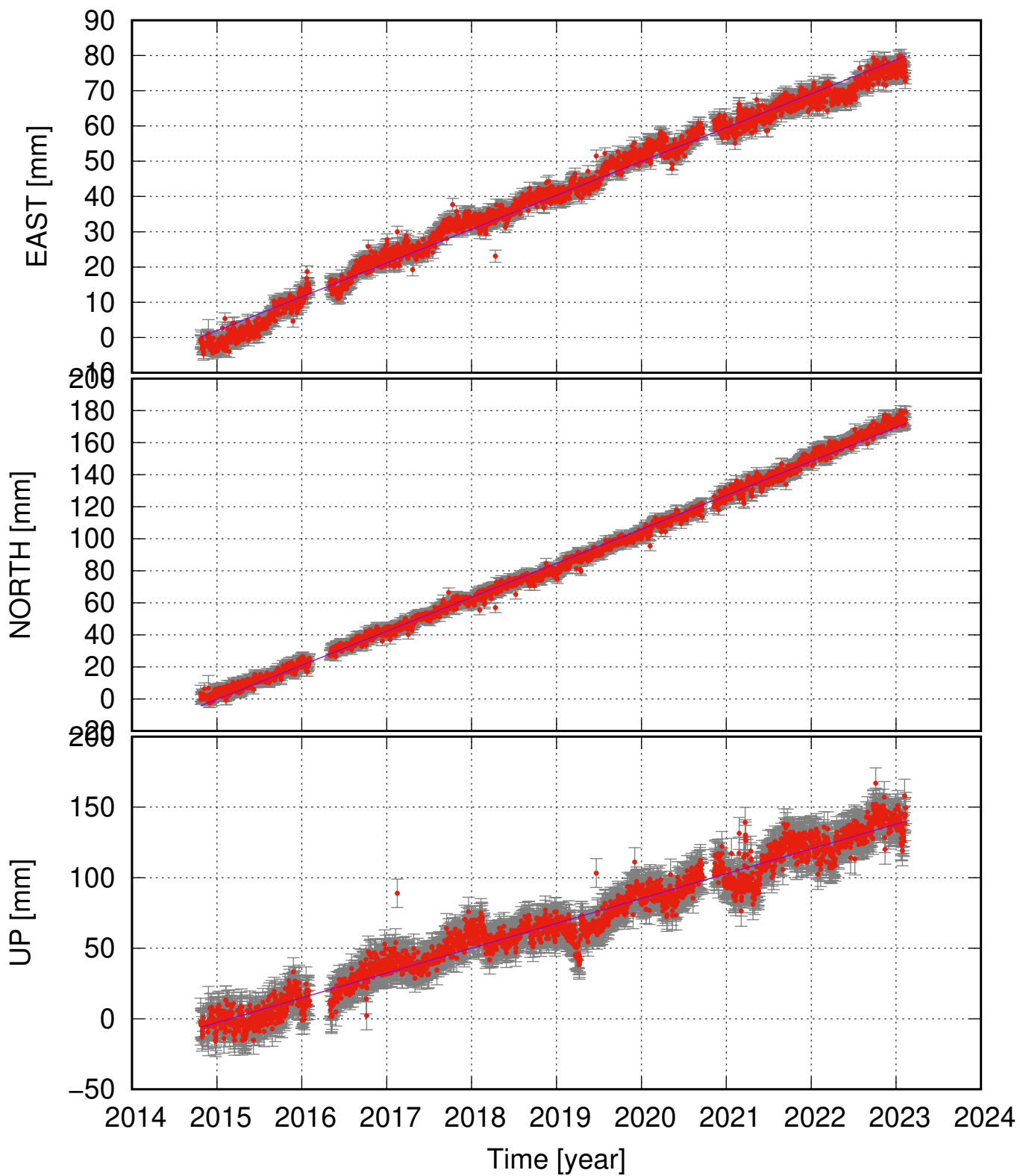
RIFC (64.92, -16.39) time series (ITRF 2014) v_e = 9.60 \pm 0.30 ; v_n = 21.21 \pm 0.35 ; v_u = 17.59 \pm 0.97 mm/yr
