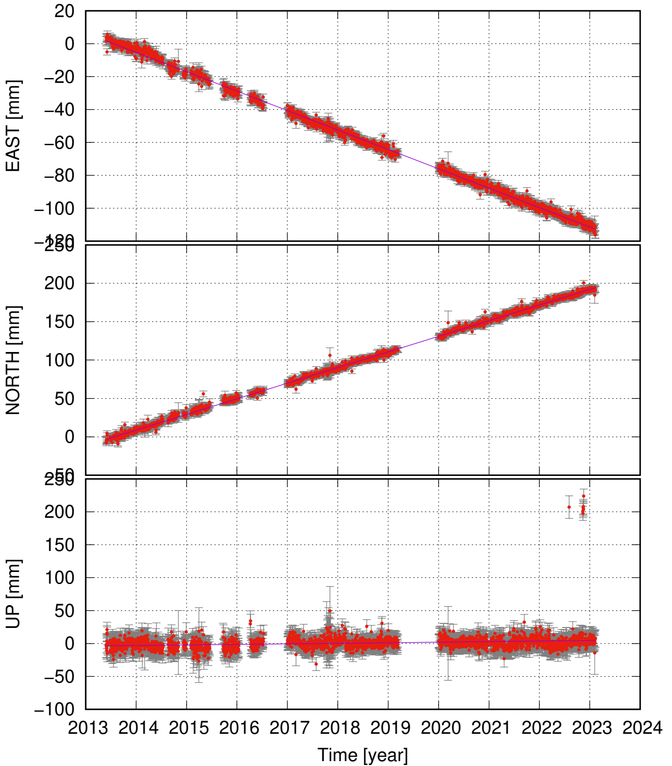
RHOL (65.43, -22.21) time series (ITRF 2014) v_e = -11.80 \pm 0.18 ; v_n = 20.36 \pm 0.24 ; v_u = 0.85 \pm 1.28 mm/yr
